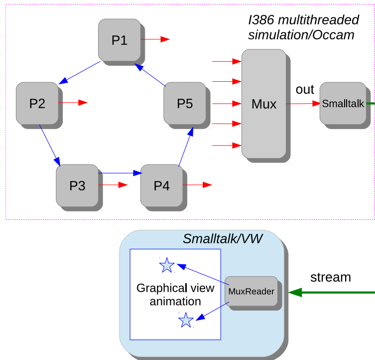
Figure 6.2: System organization between simulator and graphical interface
